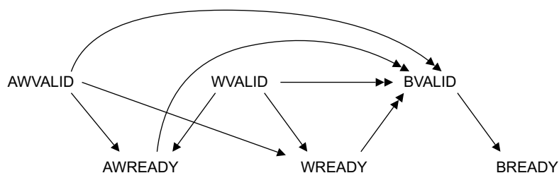
Figure 13-1 Slave write response dependencies
