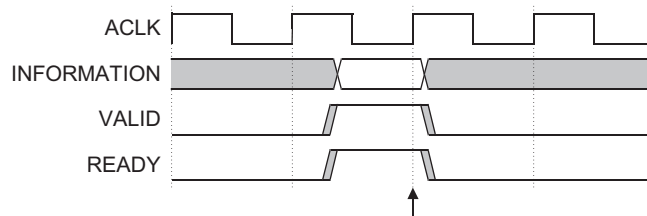
Figure 3-3 VALID with READY handshake
