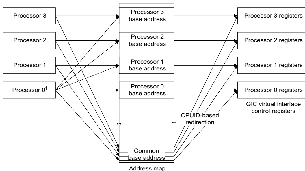
Figure 5-2 GIC virtual interface control register mappings
